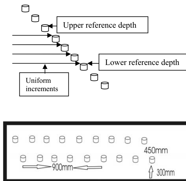
Figure 5-4 Establishment of burial depth and lane layout (not to scale)
